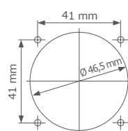
Cut-out dimensions
