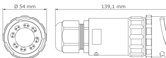
Inline male
