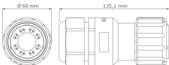
Inline female - Multiway
