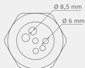
6-way
