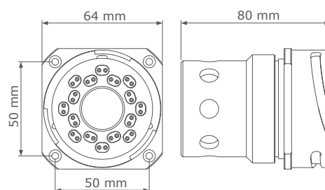
Panel male SGH 16.1 | with perforated backshell
