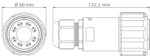
Inline female
