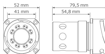
Panel male
