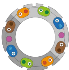
SGH 8.1 female Wiring diagram
