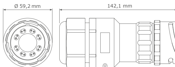
Inline male - Multiway
