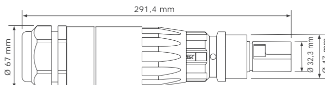
Oversized body
