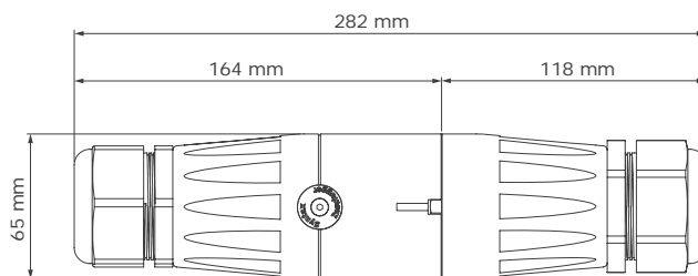
InsuLugger Slim
