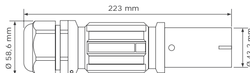
Standard body
