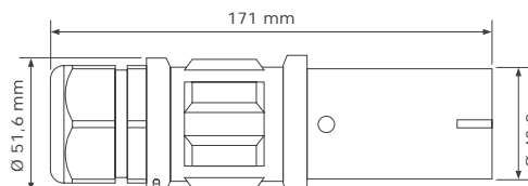
Short body
