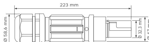
Standard body
