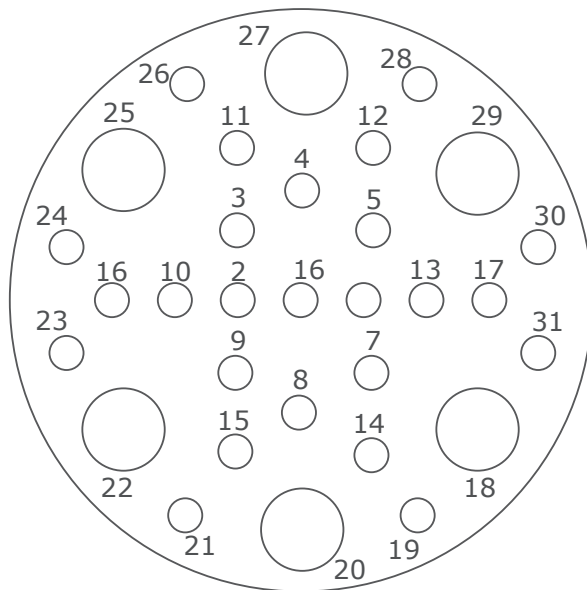
Female insert front view (SV series)
