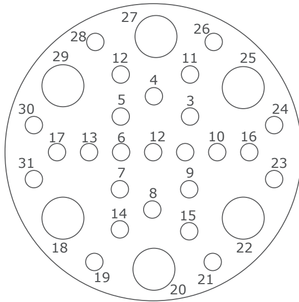
Male insert front view (SV series)
