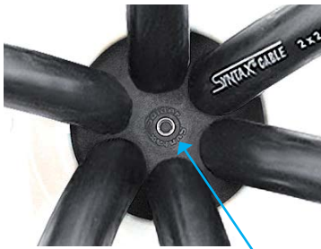
Moulded nut to insert/pull out the rubber grommet, using the removal tool
