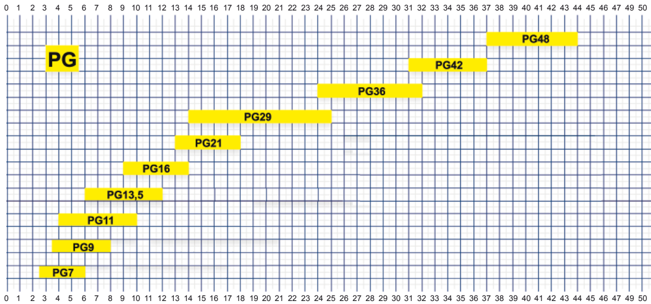
CABLE DIMENSION TO BE USED WITH PG GLANDS (MM)
