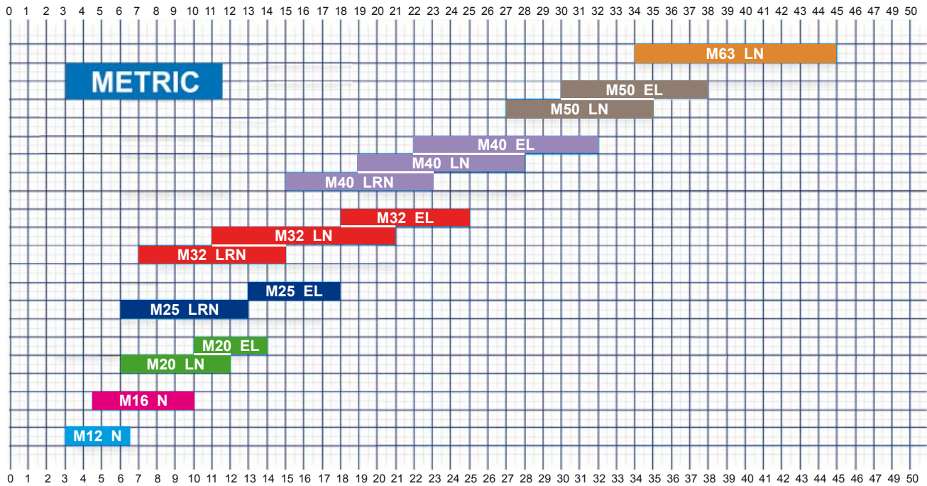
CABLE DIMENSION TO BE USED WITH METRIC GLANDS (MM)
