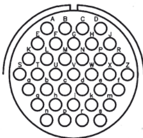
37 pin / size 28
