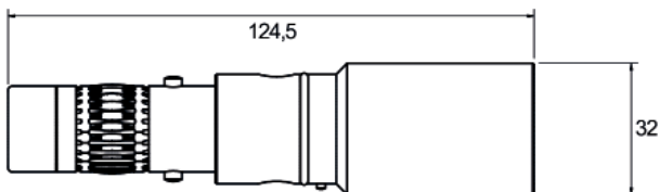
SPV 120-240 - 480amp Source contact - Crimp termination - For cable up to 240 mm 2
